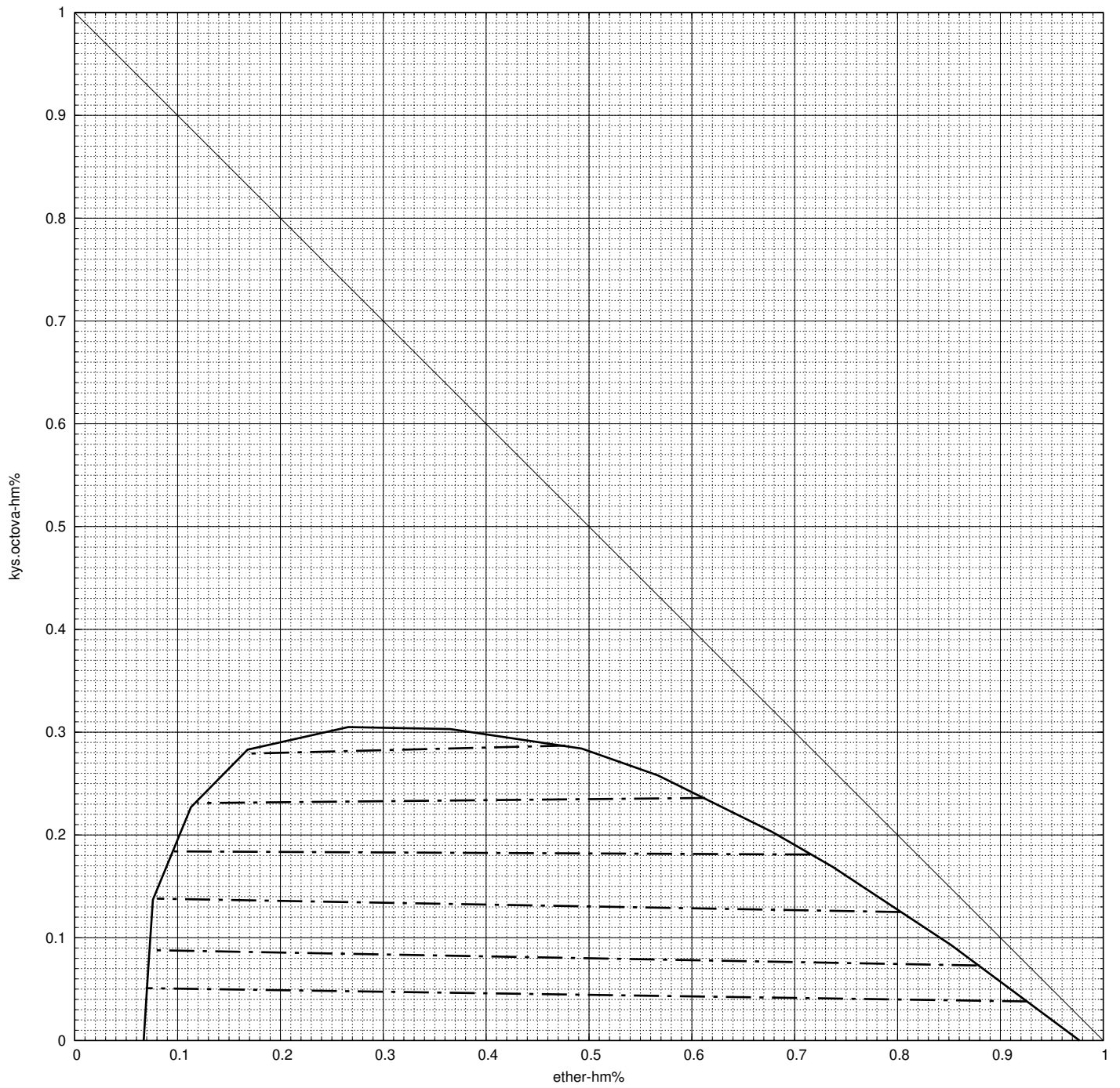
VODA-KYS.OCTOVA-DIETHYLETER (25 C)
