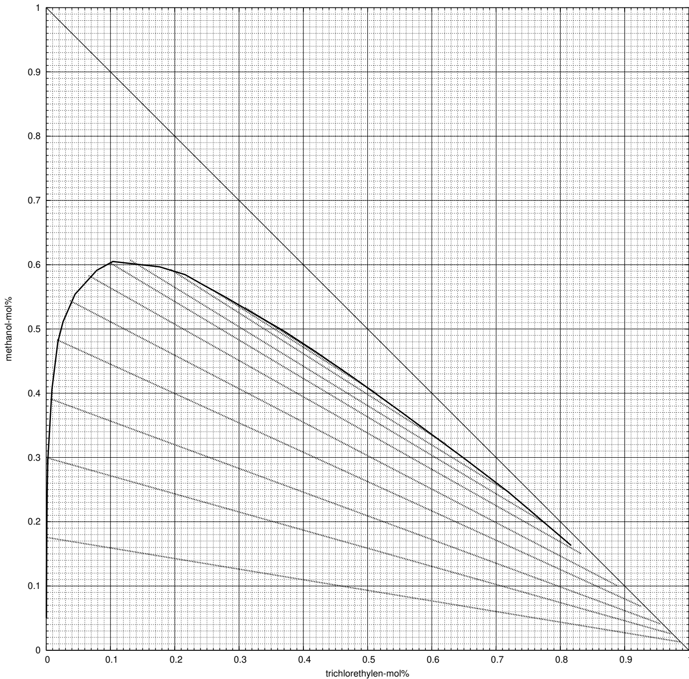
VODA-METHANOL-TRICHLORETHYLEN (20 C)
