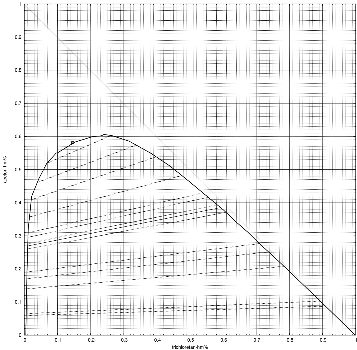
VODA-ACETON-TRICHLORETAN (25 C)
