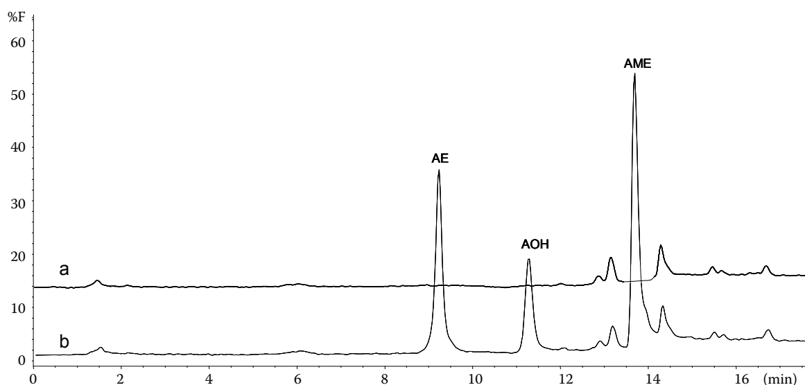
Figure 3. HPLC/FLD chromatograms of (a) blank and (b) spiked linseed sample (spiking level 100 \mu\text{g}/\text{kg} AE and 200 \mu\text{g}/\text{kg} AOH and AME, each)
