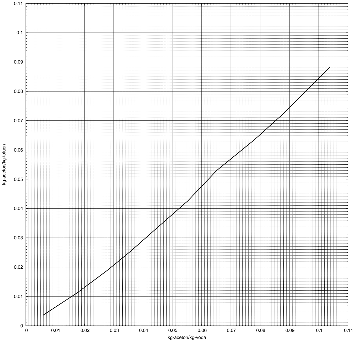
VODA-ACETON-TOLUEN (20C)
